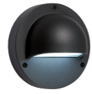
Deimos Anthracite (3095011) Warm white / White 1 W / 22 lumen Aluminium - Anthracite 80 x 140 mm (H x Ø)
